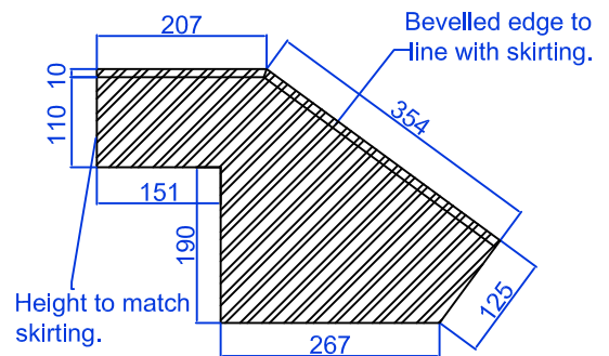
Pre-cast Terrazzo Top Stair Stringer.
