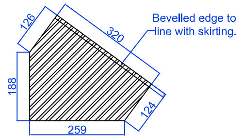
Pre-cast Terrazzo Intermediate Stair Stringer.
