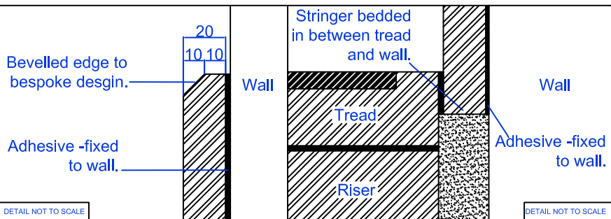
Detail A- Finished Top Edge Detail
