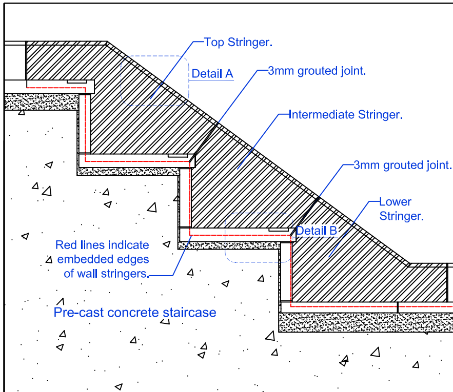
Typical Pre-cast Terrazzo Stair Section Detailing String Pieces
