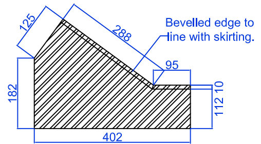
Pre-cast Terrazzo Lower Stair Stringer.
